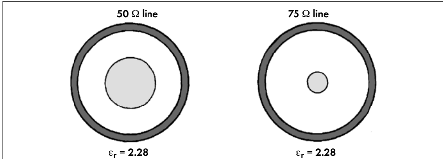
Figure 14 Different impedances caused by different insulator diameters
