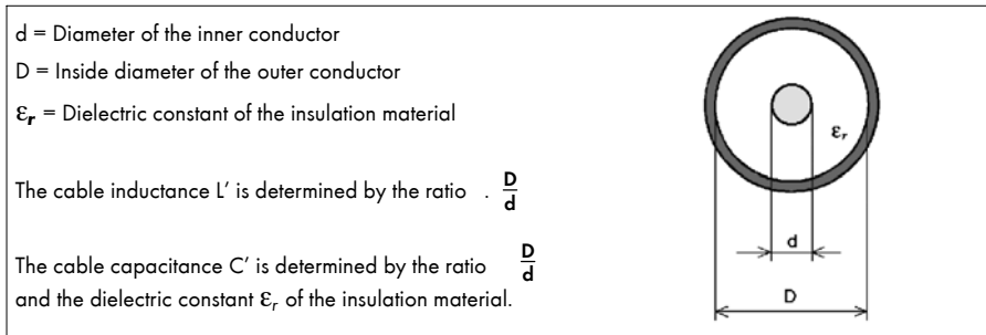
Figure 13 Diameters of inner and outer conductors
