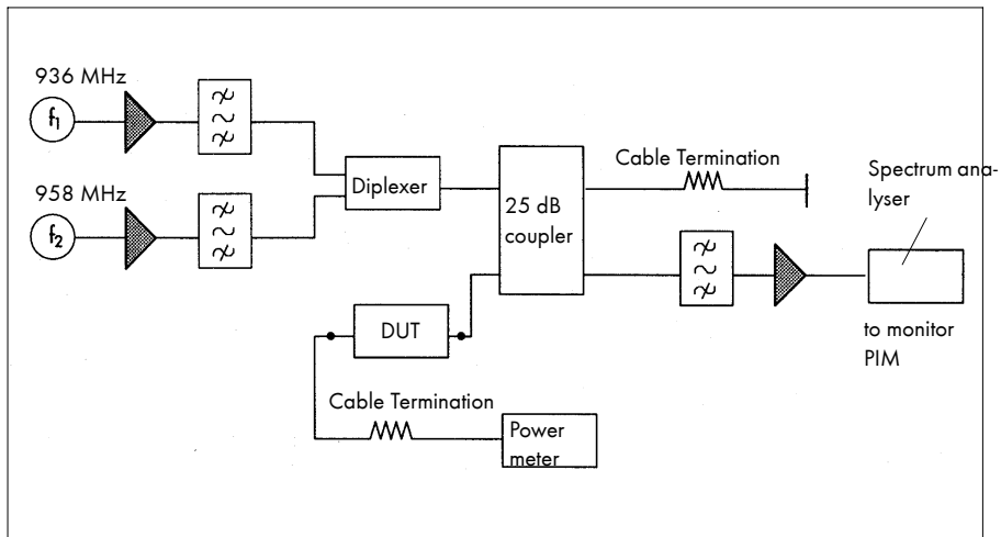
Figure 89 Schematic diagram of PIM test set-up (GSM, 900 MHz system)
