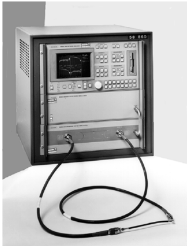
Figure 84 Photograph of test set-up No. 1 with SMA assembly
