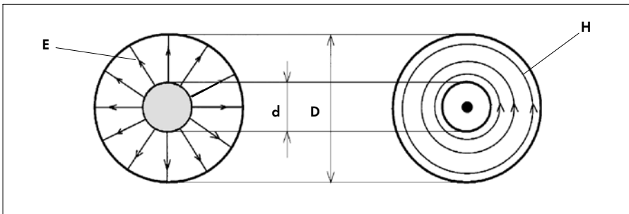
Figure 6 Cross section view: Electric and magnetic fields inside the RF line
