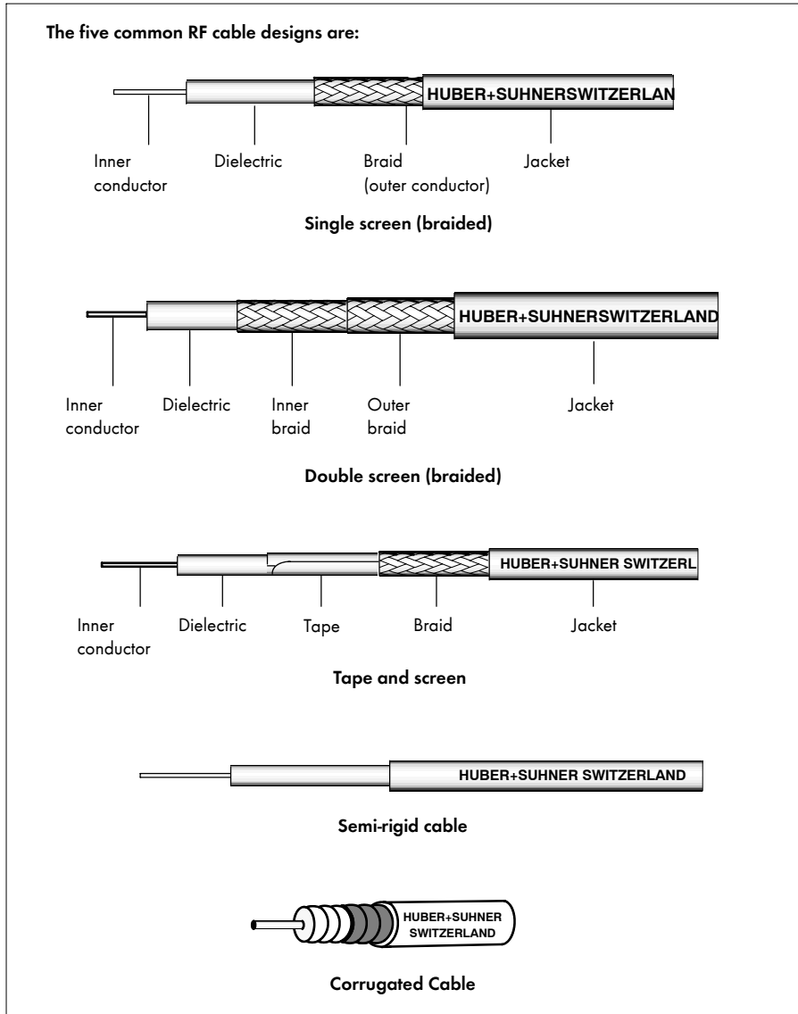
Figure 60 Cable designs
