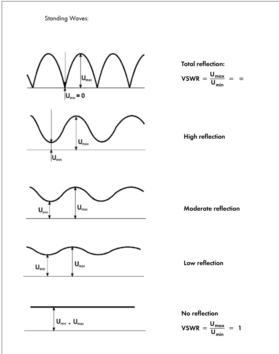
Figure 25 Various standing waves
