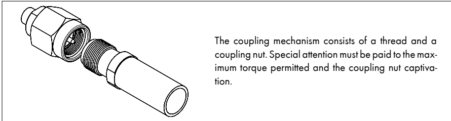
Figure 50 Threaded coupling mechanism
